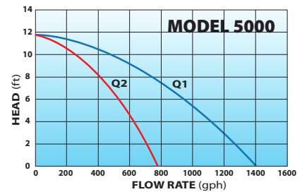
Q1: Valve Open Q2: Valve Closed Flow Rate calculated with flooded suction and no output restriction.
