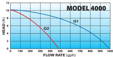
Q1: Valve Open Q2: Valve Closed Flow Rate calculated with flooded suction and no output restriction.
