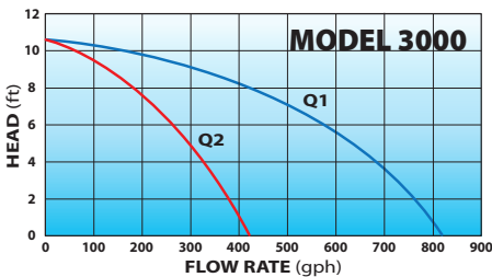
Q1: Valve Open Q2: Valve Closed Flow Rate calculated with flooded suction and no output restriction.
